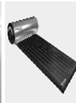
GEYSERS
